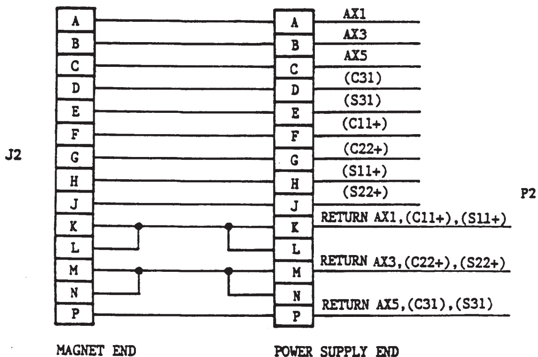
WIRING DIAGRAM S/C SHIM COIL CABLE 46-260726G1 ILLUSTRATION 2-4
