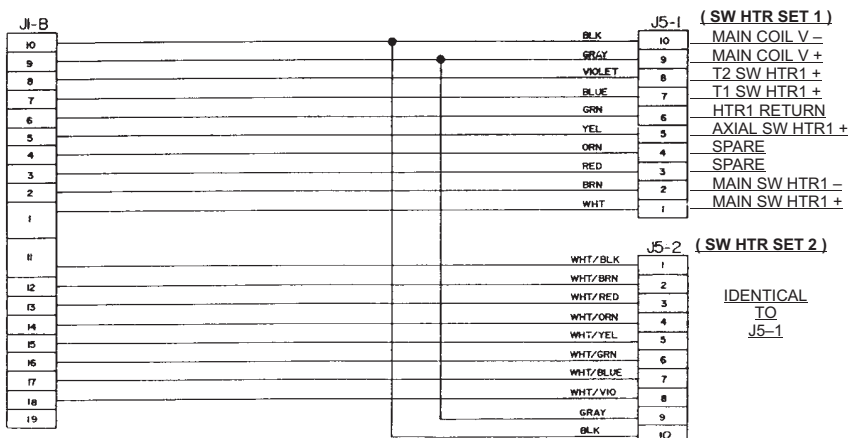
WIRING DIAGRAM MAGNET CABLE 46-260709G1 ILLUSTRATION 2-3
