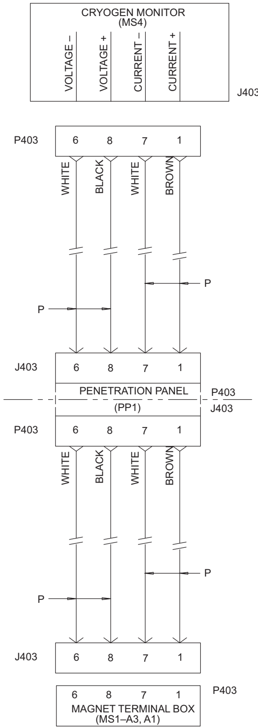
WIRING DIAGRAM LIQUID HELIUM MONITOR CIRCUIT ILLUSTRATION 2-6
